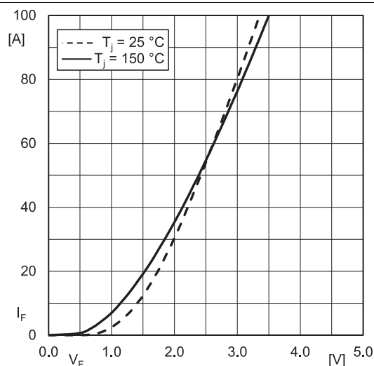
Fig. 10: Typ. Diode forward charact., incl. R CC'+EE
